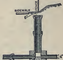
FIG. 10. HOUSE CONNECTION INSPECTION HOLE.
